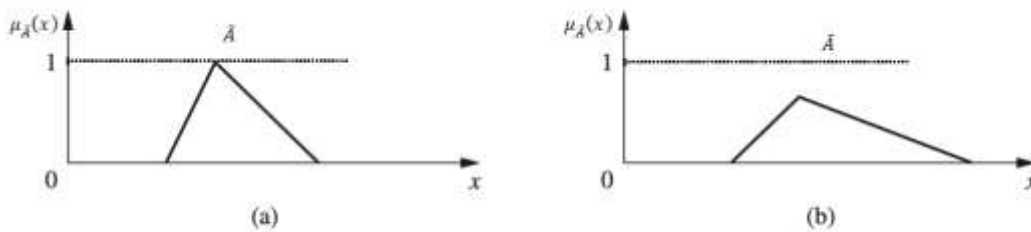
Figure 6: (a) Normal and (b) subnormal fuzzy sets.
